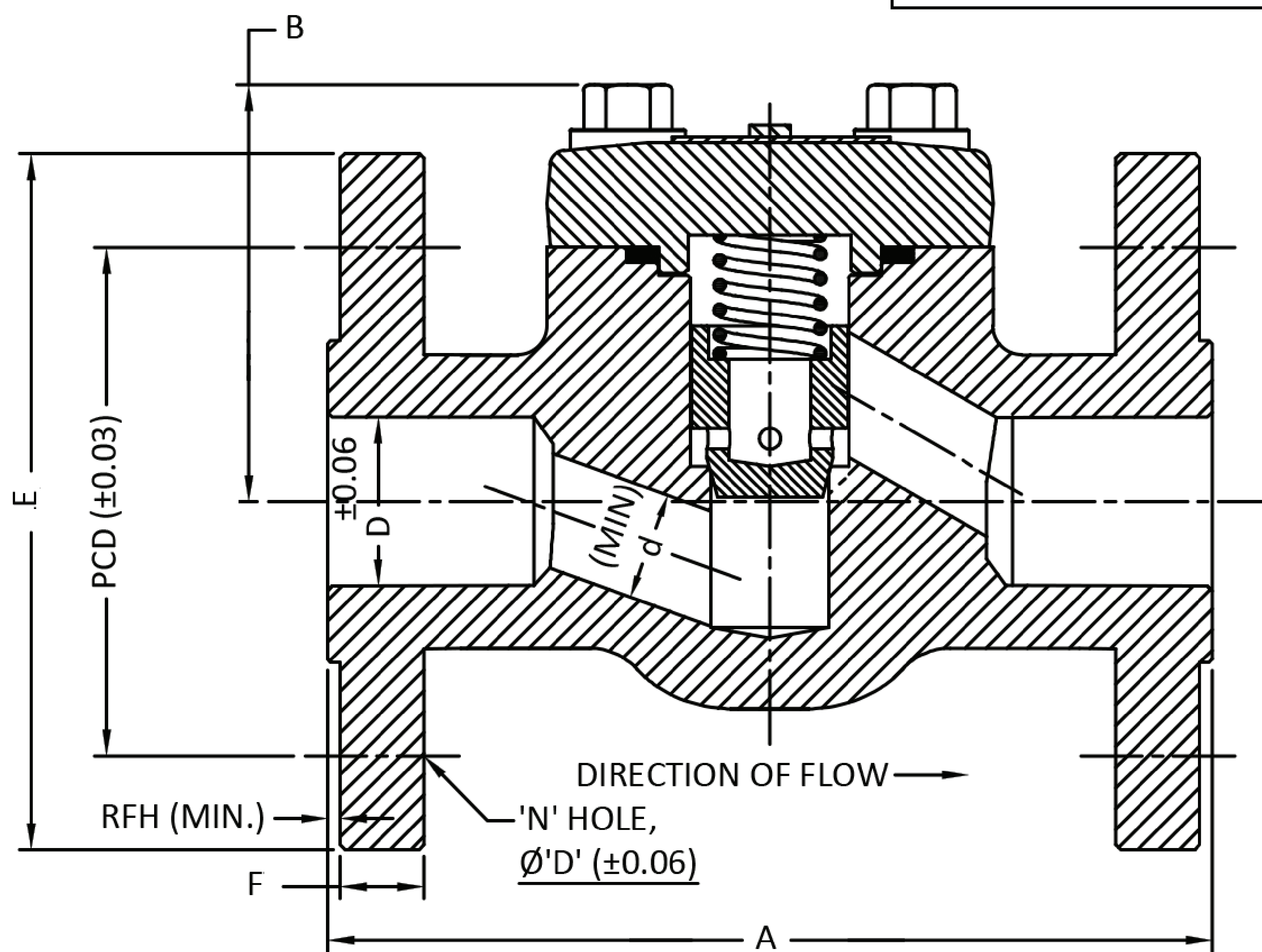
DIMENSIONS (INCHES) CLASS 150
