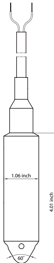
Fig. 1. Dimensional Drawing
